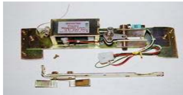
9-99-5566 L1 FAIL SECURE LOCK
