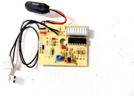
CM-DTMOD RF TRANSMITTER 318MHz FREQUENCY BOARD TRANSMITTER WIRES TO SWITCH
